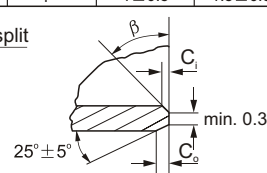
Detail z
